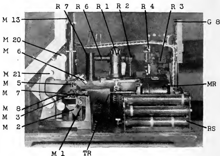
FIG. 2. Photograph of right side of graininess photometer half assembled. (The designations refer to those in Fig. 1.)
